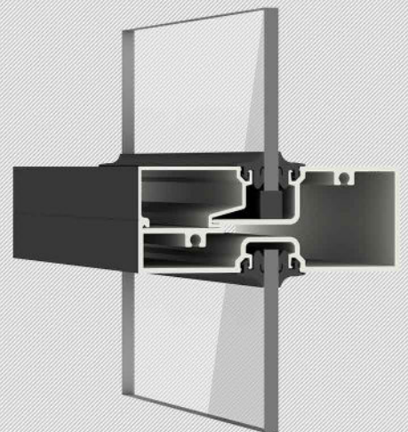
Typical Glazing Cross Section
