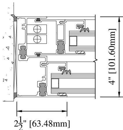
SERIES 740 SEALED UNITS WINDOW ELEVATION WITH SIDELITE
